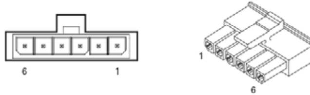
FIGURE 9. Motor sensor connector used for SSI Encoders
