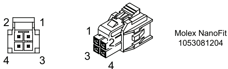
FIGURE 14. STO Connector Pins Identification
