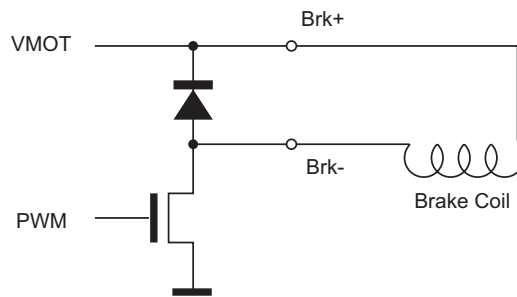
FIGURE 4. Mechanical Brake internal drive circuit and connection
