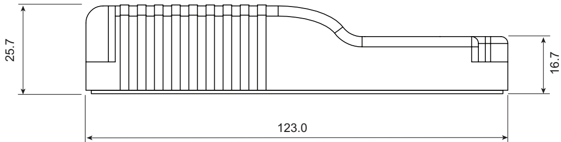
FIGURE 12. SDC3260 Side View and Dimensions
