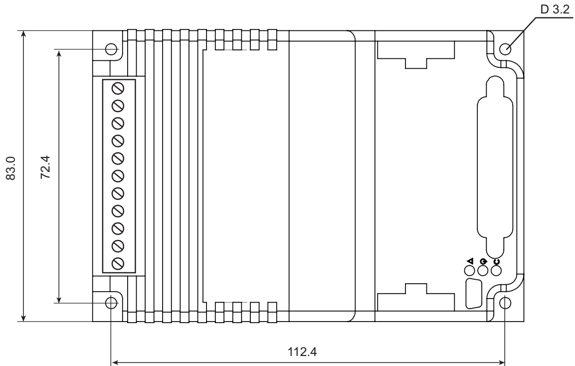
FIGURE 13. SDC3260 Top View and Dimensions
